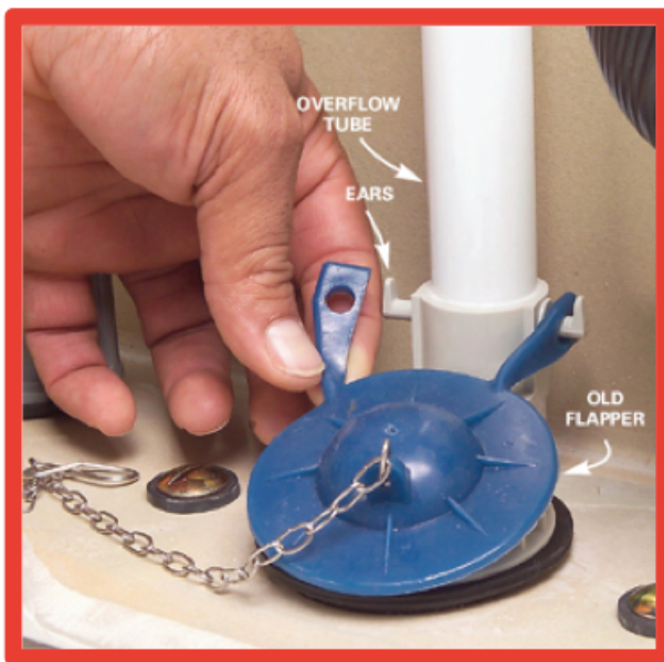
Remove Leaky Flapper
